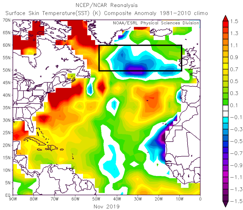
Figure 5: November 2019 SST anomalies across the North Atlantic Ocean. The black box highlights the region where SSTs are measured for the CSU AMO index.
