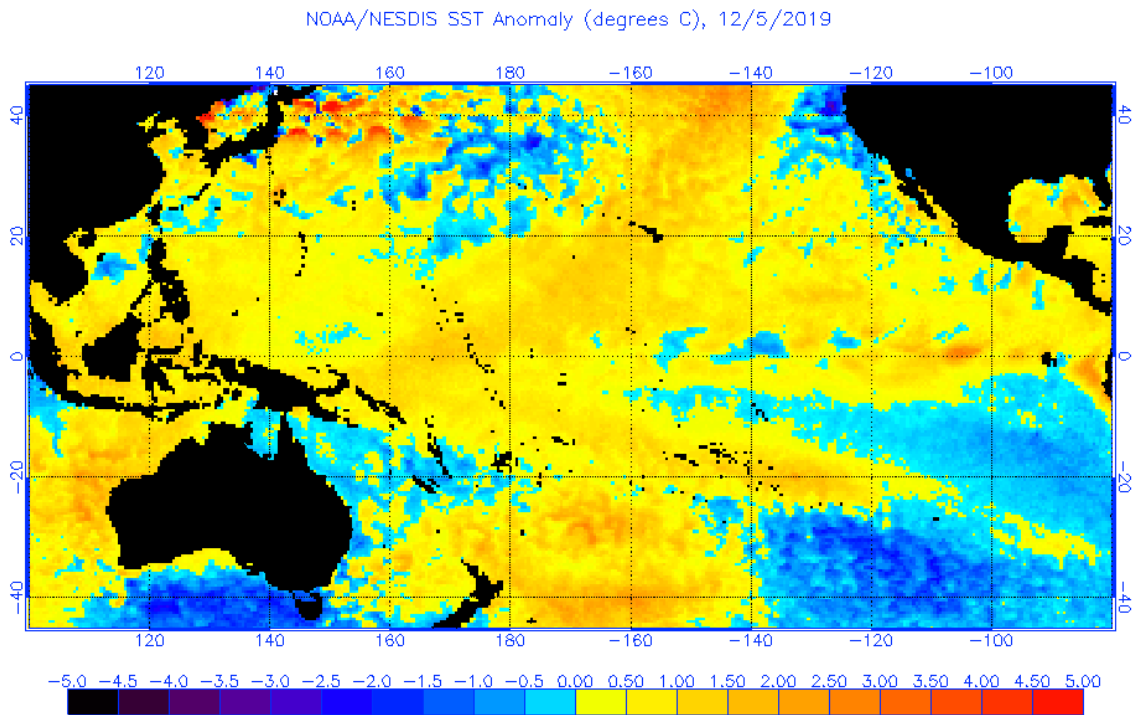
Figure 6: Early December 2019 SST anomalies across the Pacific Ocean. Warm SSTs prevail across the entire tropical Pacific at the present time.
