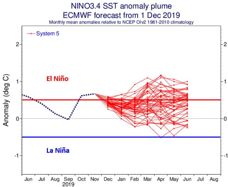
Figure 8: Ensemble ECMWF forecast plume for Nino 3.4 SSTs over the next few months. Most ECMWF ensemble members predict neutral ENSO conditions through next spring.
