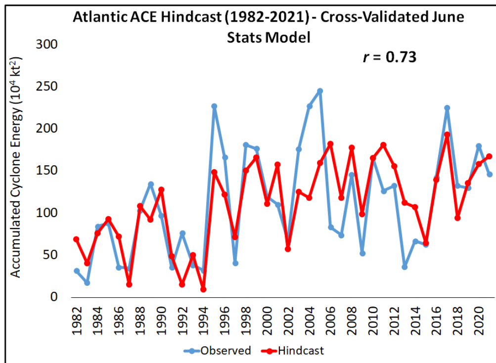
Figure 1: Observed versus early June cross-validated hindcast values of ACE for the statistical model for 1982–2021.
