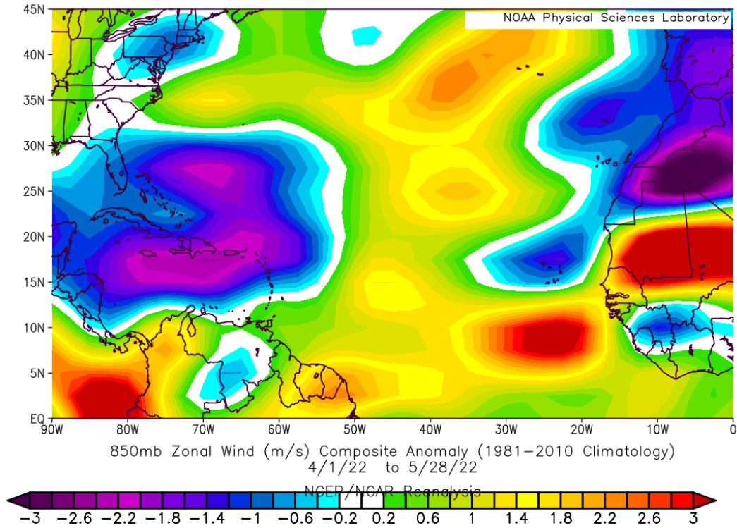
Figure 25: April 1, 2022 through May 28, 2022 averaged 850-hPa zonal wind anomalies across the North Atlantic. In general, low-level trade winds have been weaker than normal (e.g., westerly wind anomalies) across most of the tropical Atlantic over the past two months.
