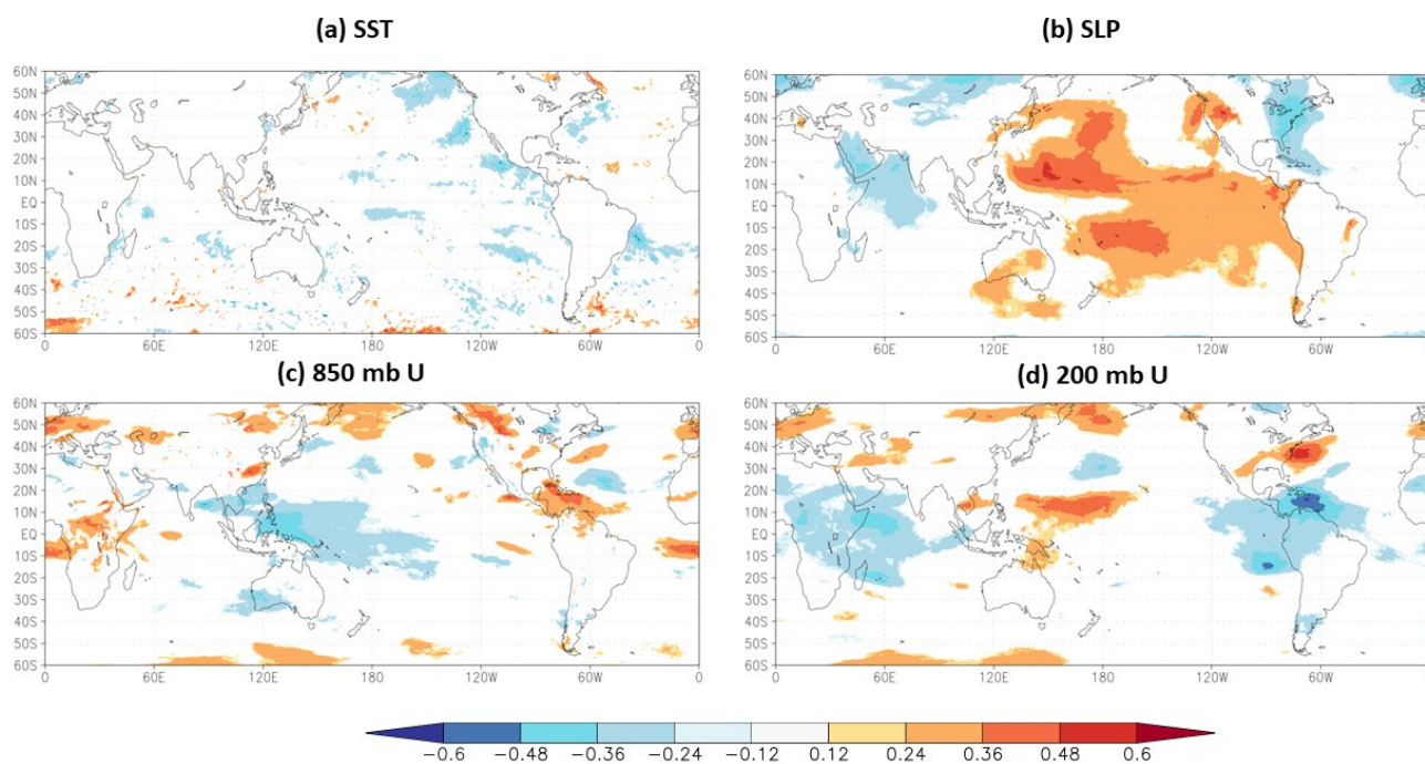
Figure 5: As in Figure 4 but for May SLP in the subtropical North Atlantic. The sign of Predictor 2 has been flipped for easy comparison with Figure 4.
