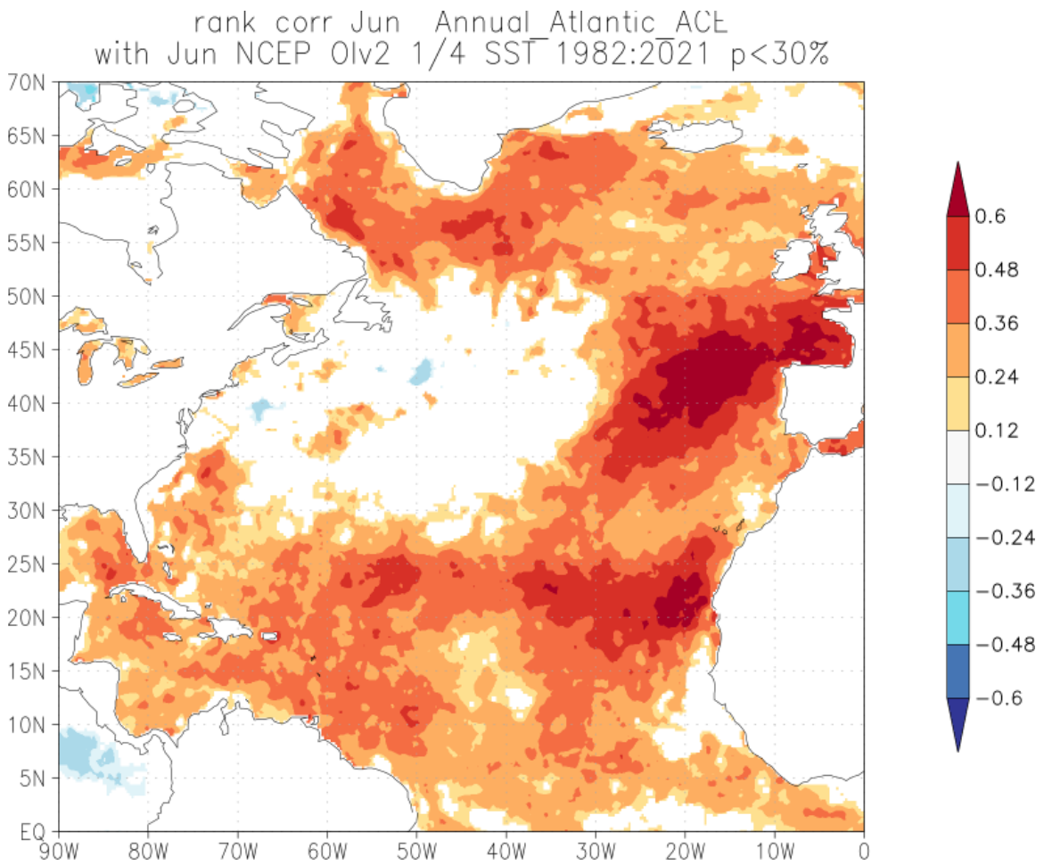
Figure 24: Rank correlation between June North Atlantic SST anomalies and seasonal Atlantic ACE from 1982–2021.
