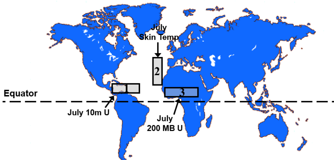
Figure 8: Location of predictors for our early June statistical/dynamical extended-range statistical prediction for the 2022 hurricane season. This forecast uses dynamical model predictions from ECMWF, the UK Met Office and JMA to predict July conditions in the three boxes displayed and uses those predictors to forecast ACE.
