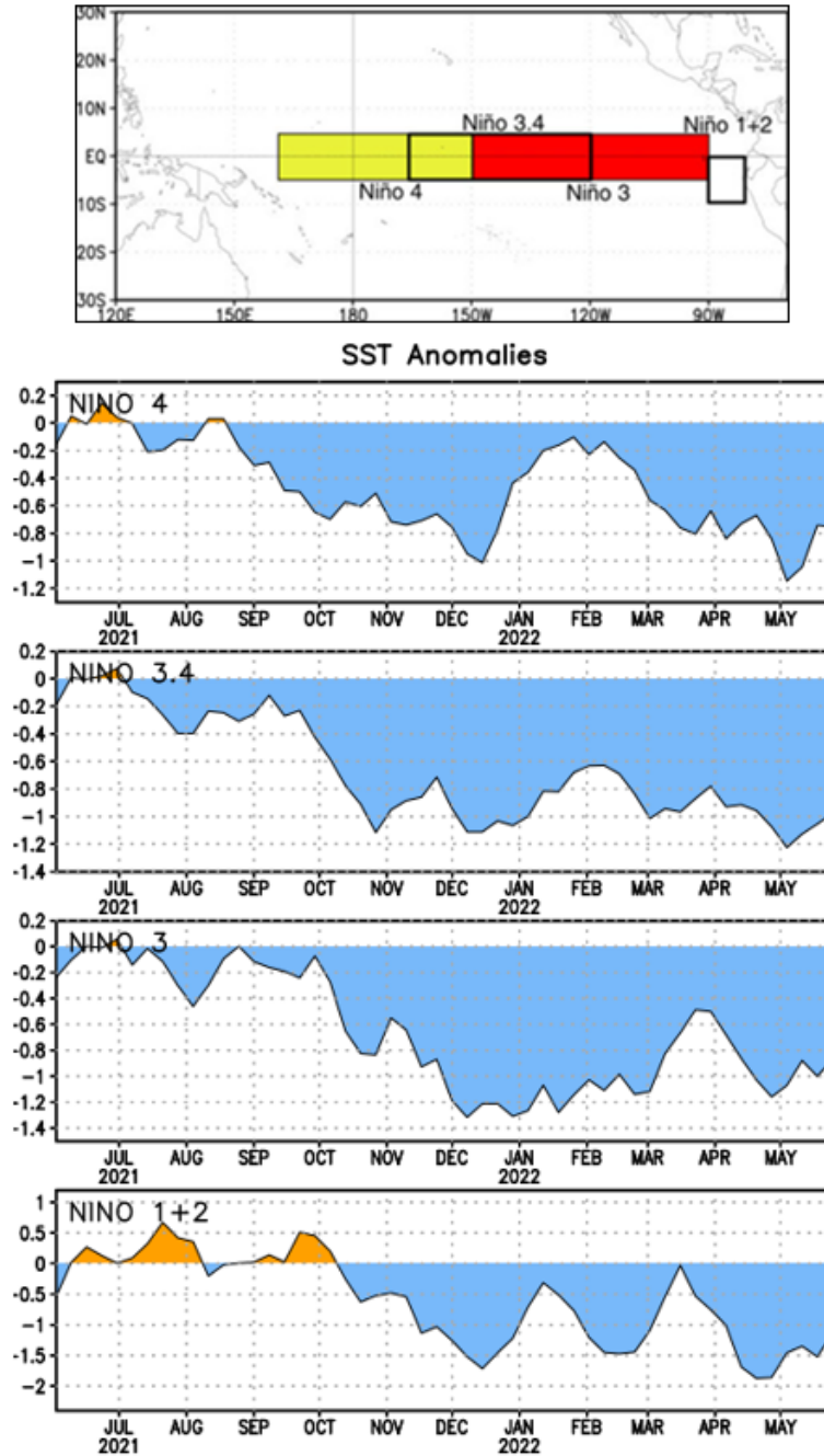
Figure 15: ENSO SST anomalies from June 2021 through May 2022. Figure courtesy of Climate Prediction Center.
