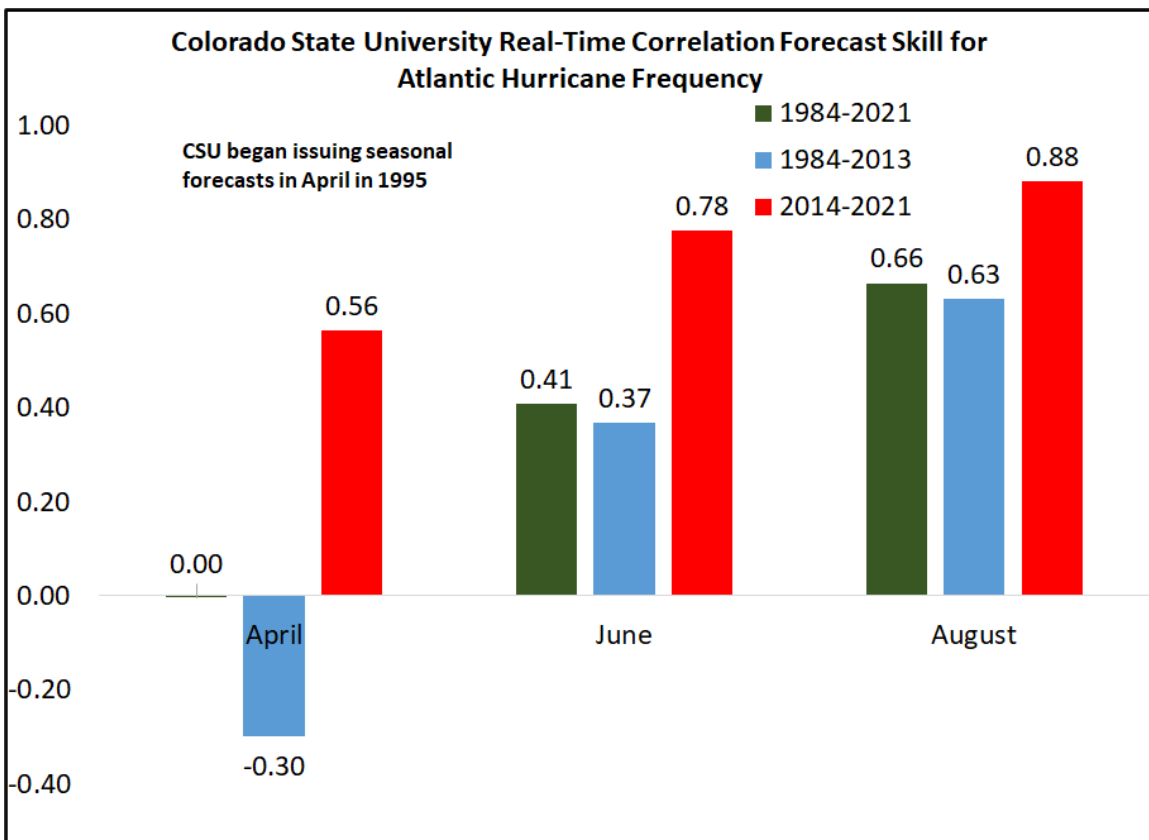
Figure 28: CSU’s real-time forecast skill for Atlantic hurricanes using correlation as the skill metric. Correlation skills are displayed for three separate time periods: 1984–2013, 2014–2021 and 1984–2021, respectively.
