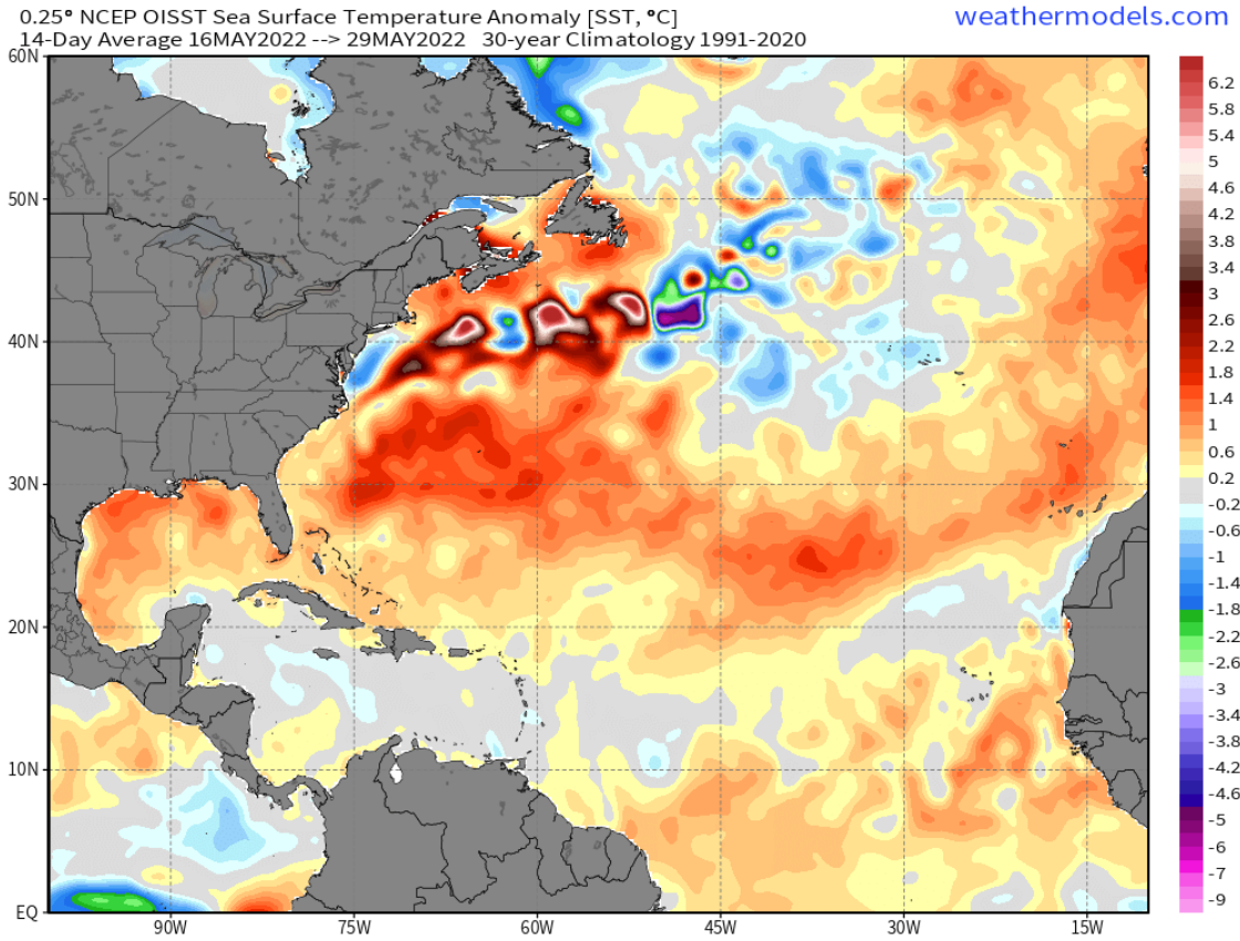
Figure 23: Late May 2022 SST anomaly pattern across the Atlantic Ocean.
