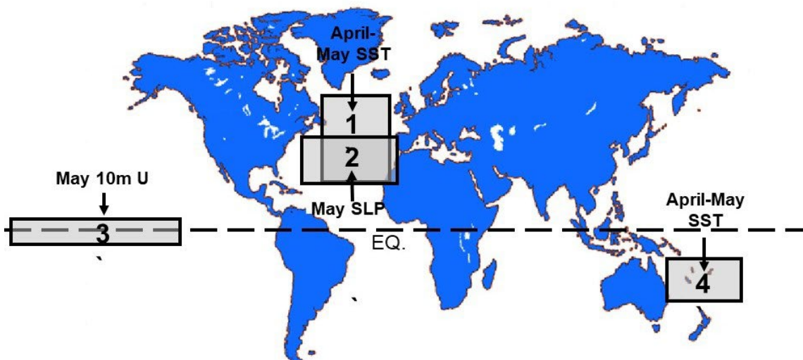
Figure 2: Location of predictors for our early June extended-range statistical prediction for the 2022 hurricane season.
