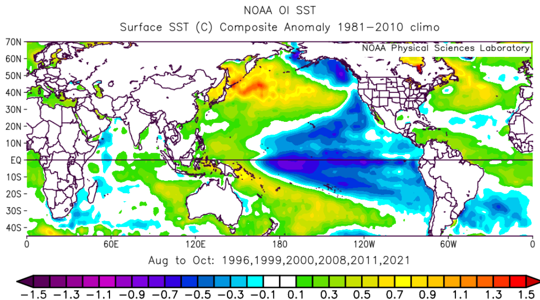
Figure 12: Average SST anomalies in our six analog years.
