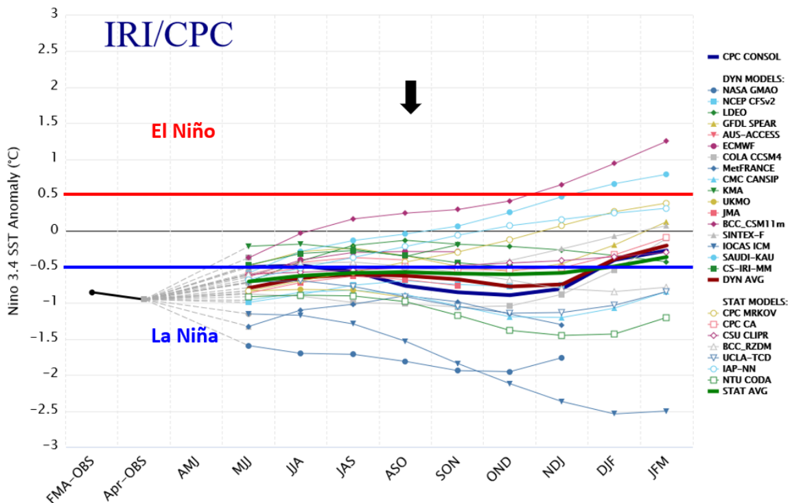
Figure 21: ENSO forecasts from various statistical and dynamical models for Nino 3.4 SST anomalies based on late April to early May initial conditions. All models are calling for either La Niña or ENSO neutral conditions for August–October. Figure courtesy of the International Research Institute (IRI). The black arrow denotes August–October – the peak of the Atlantic hurricane season.
