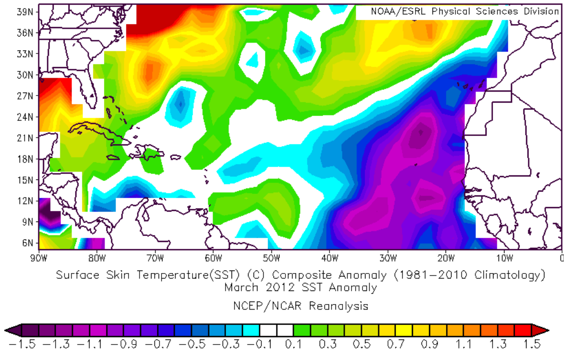
Figure 12: March 2012 SST anomaly pattern across the Atlantic Ocean.
