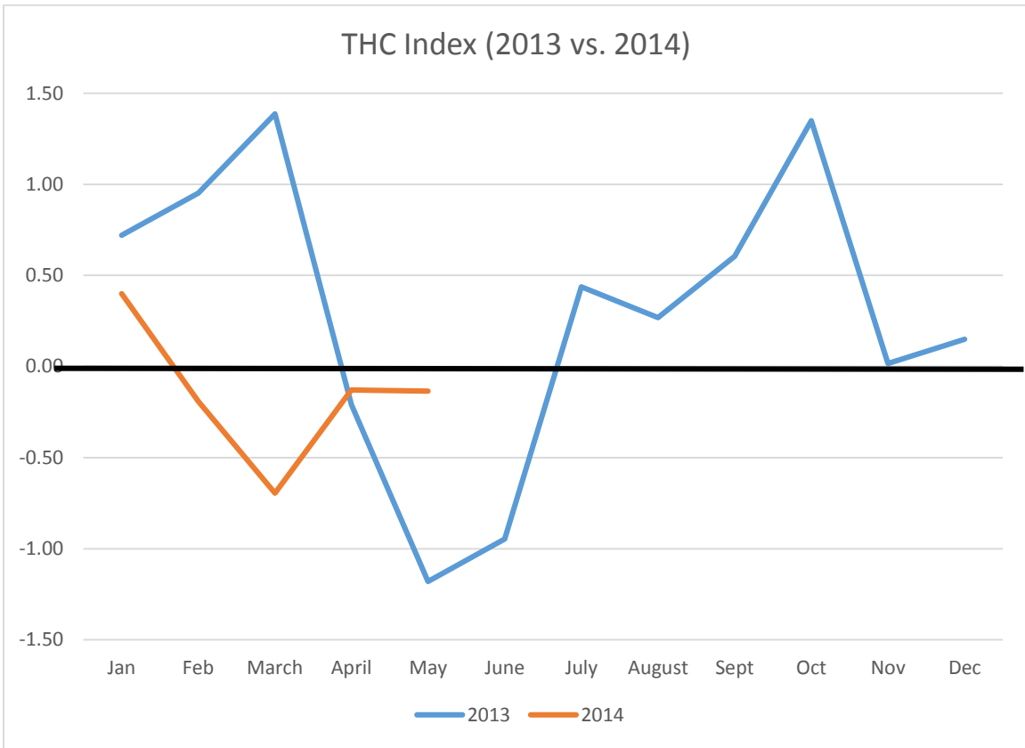
Figure 17: Standardized values of the THC/AMO index by month in 2013 and 2014. Month-to-month changes have been much less in 2014 than they were in 2013.
