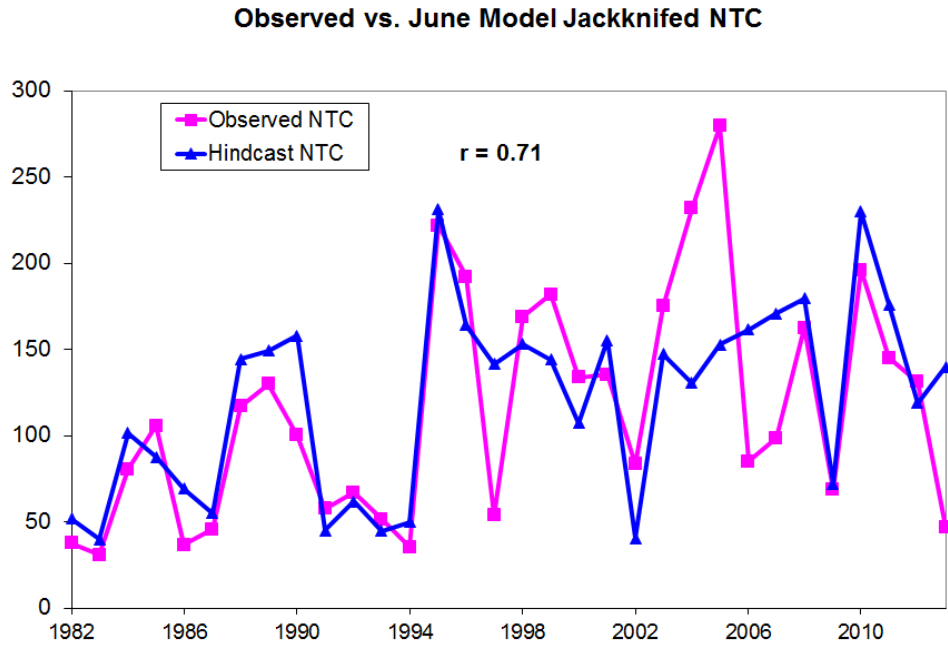
Figure 1: Observed versus early June jackknifed hindcast values of NTC for 1982-2013. The hindcast model explains approximately 50% of the variance from climatology.
