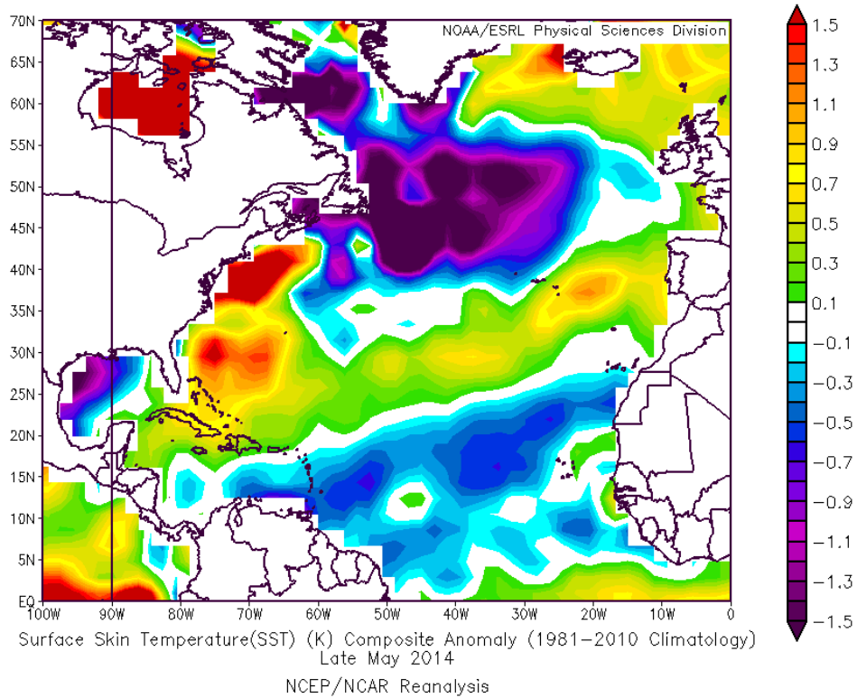
Figure 13: Late May SST anomalies across the Atlantic.
