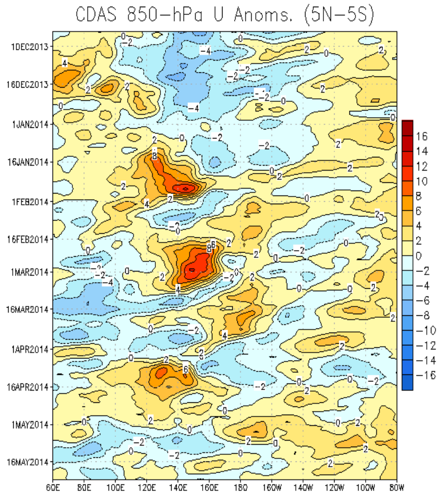
Figure 11: Anomalous low-level winds across the tropical Pacific since late November 2013. Note the areas of strong westerly wind anomalies in late January, late February and mid April near 150°E. This anomalously strong westerly wind flow drives eastward-propagating Kelvin waves associated with basinwide warming.
