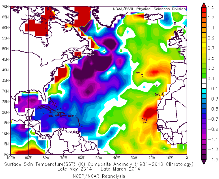
Figure 14: Anomalous SST change from late March to late May 2014.
