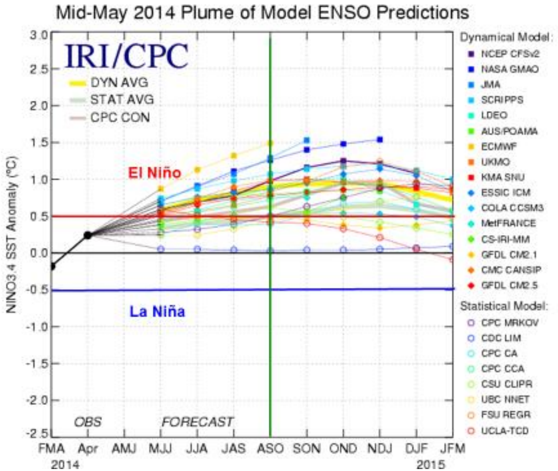
Figure 9: ENSO forecasts from various statistical and dynamical models. Figure courtesy of the International Research Institute (IRI). Most models call for warm ENSO conditions over the next several months.
