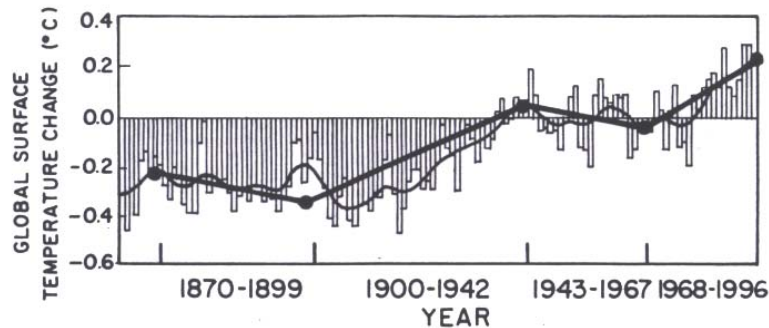
Figure 2: Portrayal of four multi-decadal time periods with different conveyor belt strengths, Sahel rainfall, Atlantic hurricane activity and frequent major El Nino events, and global surface temperature tendency.
